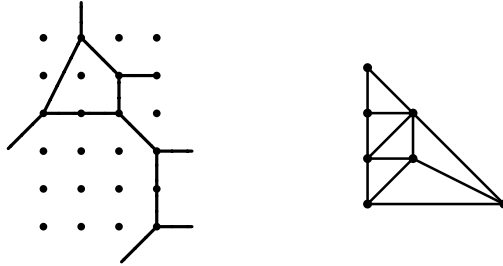
FIGURE 4. The tropicalization of C_f and its dual Newton subdivision
