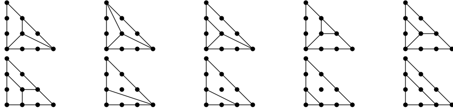
FIGURE 3. Classification of the rays of the secondary fan of \mathcal{A}_c
